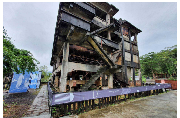
Figure 4. The remains of the coal preparation plant at the New Pingxi Coal Mine. This special exhibition allows the visitors to interact with these mining sites through installation art and equipment identification activities, guiding them to recognize the mining equipment of the past.
